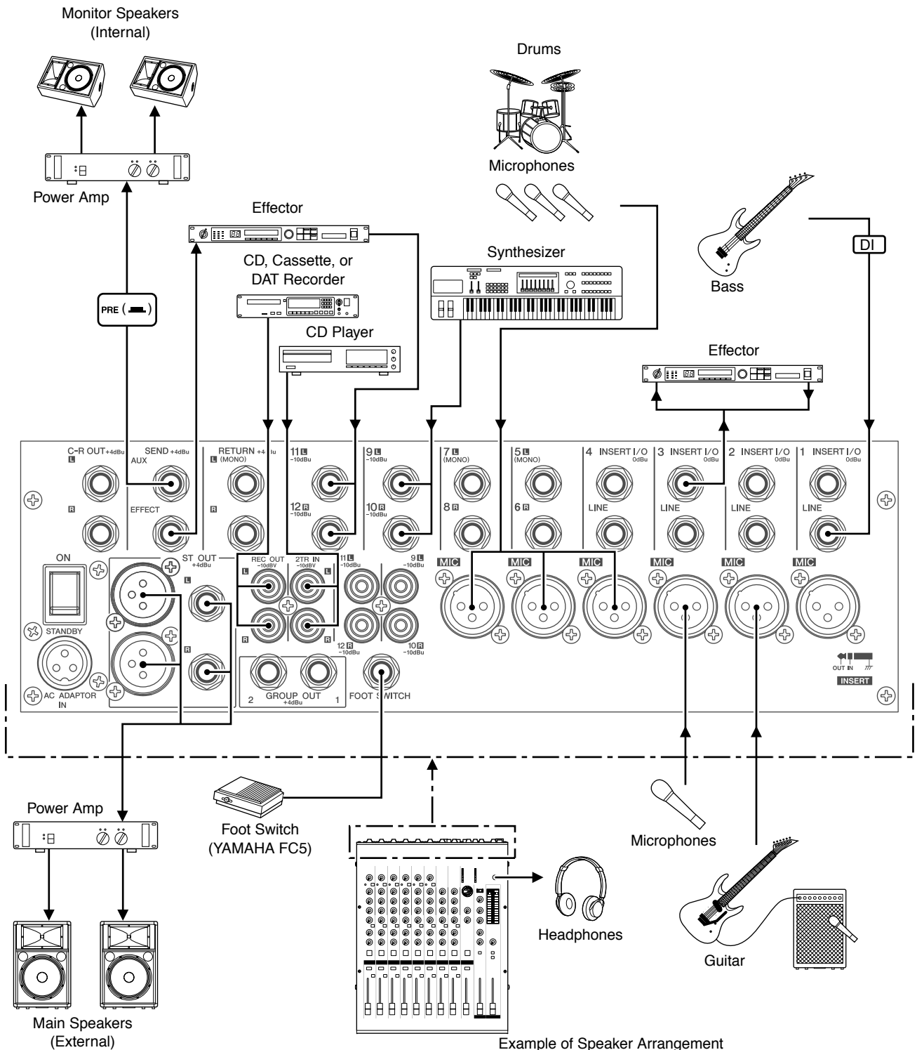
Example of Speaker Arrangement
