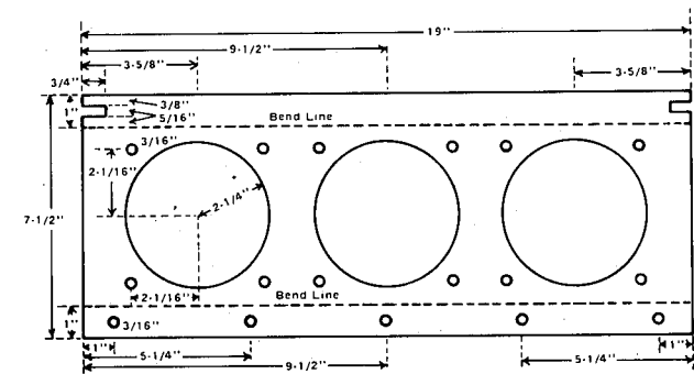
Front fan panel view before folding.
